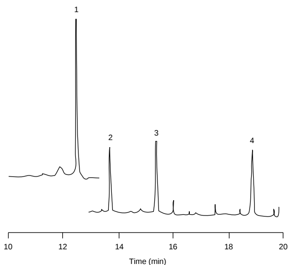
Figure 1-22. Electropherogram of four model proteins using the charge reversal system depicted in Figure 1-21. Buffer: 0.01 M phosphate, pH 7.0 with 50 \mu\text{g/mL} FC-134 added. Peak identification: (1) myoglobin (run separately); (2) ribonuclease A; (3) cytochrome C; (4) lysozyme. Reproduced with permission from Emmer et al., J. Chromatogr. 547, 544 (1991).
