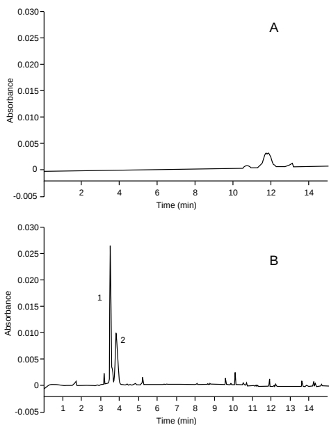
Figure 1-24. SDS-containing run buffer for the separation of glycosylated and nonglycosylated proteins. Capillary, 50- \mu m i.d. \times 27-cm length; wavelength, 200 nm; proteins, streptavidin (peak 1) and avidin (peak 2) stocks made 1 mg/mL each in 25% phosphate-buffered saline (PBS). (A) Run buffer, 500 mM sodium borate, pH 8.5; sample preparation, diluted 1:3 in water for analysis; voltage, 0- to 10-kV linear ramp over 20 min, normal polarity (toward cathode). (B) Run buffer, 200 mM sodium phosphate, pH 2.0, 0.1% SDS; sample preparation, stocks diluted 1:3 in 1% SDS, 5% 2-mercaptoethanol, 2.5 mM Tris-glycine (pH 8.9), 10% glycerol, and boiled for 5 min; voltage, 10 kV, constant, reverse polarity (toward anode). Reprinted with permission from Palmieri and Nolan, Handbook of Capillary Electrophoresis , Landers (Ed.), Boca Raton: CRC Press, 1994.
