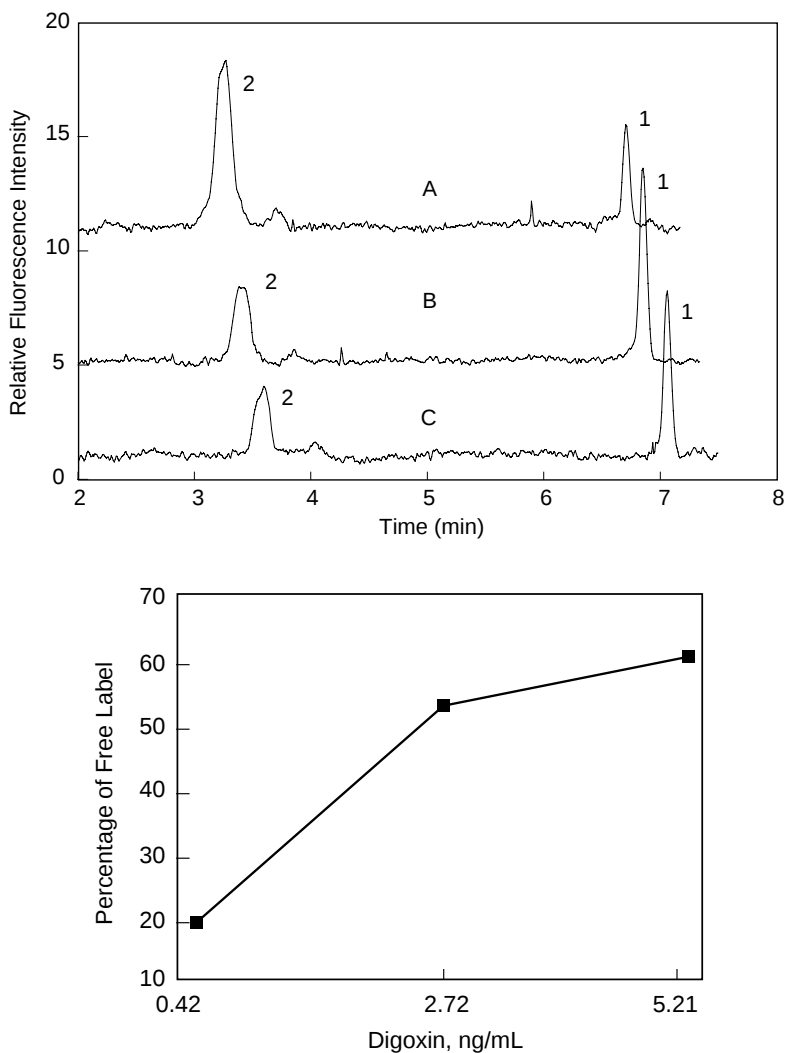
Figure 2-14. (Top) Digoxin immunoassay with serum calibrator at (A) 0.42, (B) 2.72 and (C) 5.21 ng/mL, respectively. Peaks: 1, digoxigenin-3'-(dT) 10 -TMR; 2, antigen-antibody complex of the Fab. (Bottom) Calibration curve. Percentage of free digoxigenin-3'-(dT) 10 -TMR vs. digoxin calibrates. Reproduced with permission from Chen and Sternberg, Electrophoresis 15, 13 (1994).
