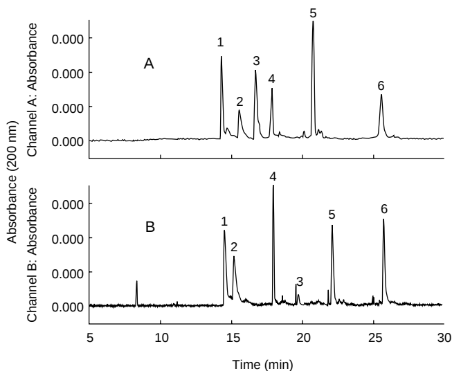
Figure 1-18. Effect of zwitterionic additive (O-phosphorylethanolamine) on separation efficiency. (A) run buffer, 250 mM sodium phosphate, pH 6.0; (B) 100 mM sodium phosphate, plus phosphorylethanolamine, pH 5.8. Peak identification: (1) lysozyme; (2) cytochrome C; (3) EOF marker; (4) myoglobin; (5) carbonic anhydrase; (6) \beta -lactoglobulin A. Reproduction with permission from Chen et al., J. Liq. Chromatogr. 15, 1143 (1992).
