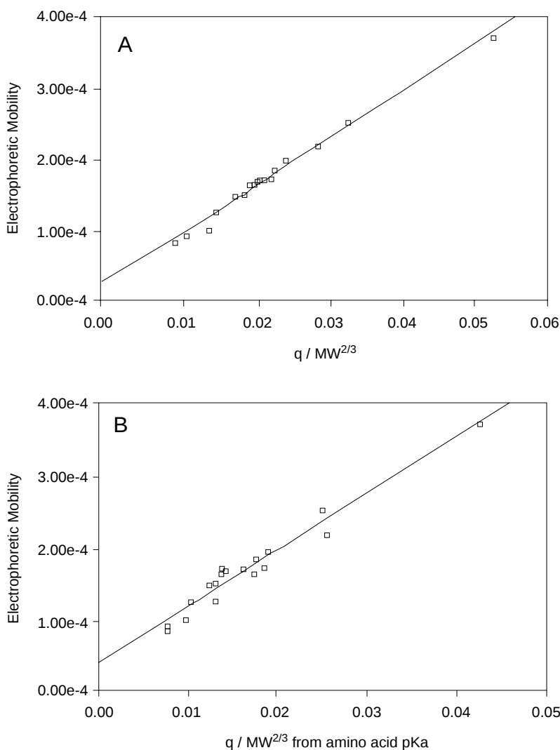
Figure 1-2. Fit of electrophoretic mobility ( \text{cm}^2/\text{V}\cdot\text{s} ) versus the charge-to-size parameter for hGH digest separated in 0.1 M glycine, pH 2.35. (A) Data from pK_a values calculated at Eli Lilly. Correlation coefficient, 0.989. (B) Data based on pK_a values of the isolated amino acids. Correlation coefficient, 0.956. Data reproduced with permission from Rickard et al., Anal. Biochem. 197, 197 (1991).
