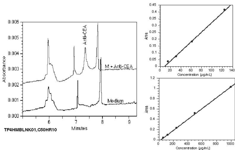
Figure 2-12. CZE analysis of anti-CEA MAb in tissue culture. Capillary, eCAP Neutral coated, 37 (30) cm \times 50 \mu m; run buffer, 20 mM citrate pH 3; run temperature, 20 ^{\circ} C; field strength, 400 V/cm; detection, 214 nm.
