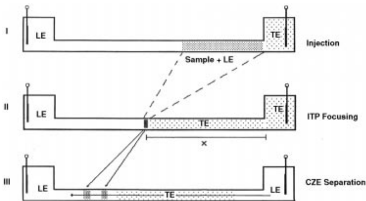
Figure 1-30. Schematic illustration of transient ITP sample preconcentration in CE. Method A: replacement of the terminating electrolyte. From: Foret et al. , Beckman Technical Information Bulletin A-1740 (1993).
