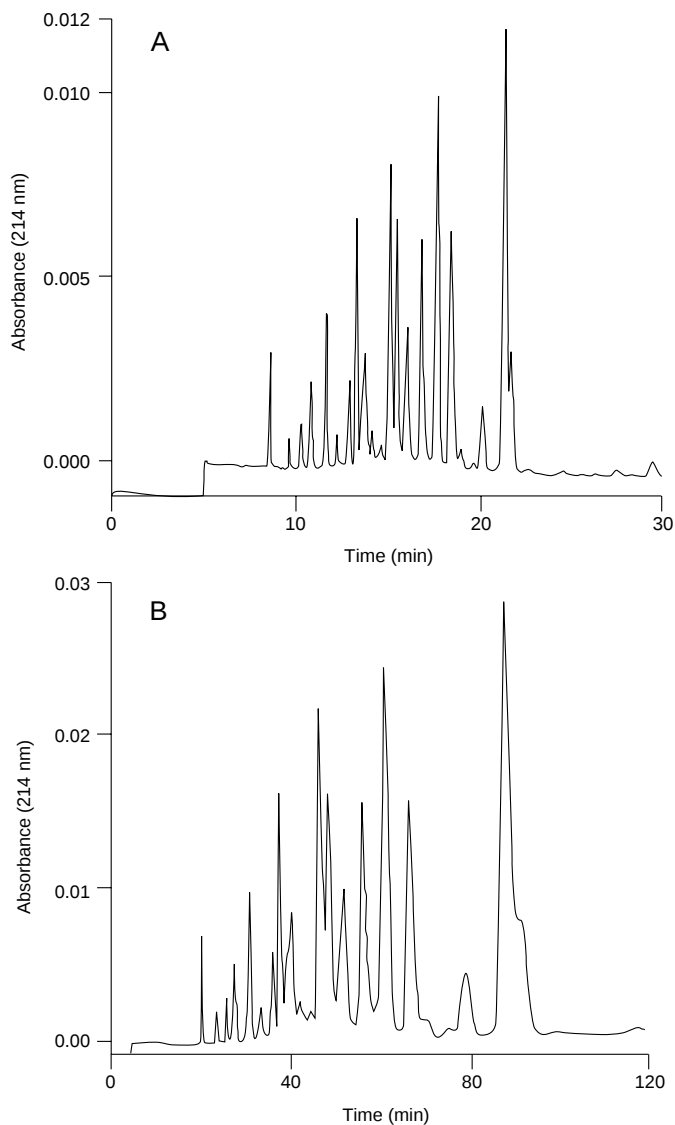
Figure 1-40. Comparison of analytical and micropreparative CE of a \beta -lactoglobulin tryptic digest. (A) analytical CE with a 75- \mu m-i.d. capillary. (B) micropreparative CE with a 200- \mu m-i.d. capillary. See text for details. From Smith and Ohms, Techniques in Protein Chemistry III (1992).
