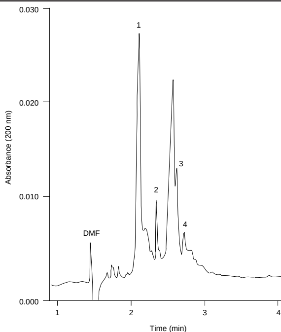
Figure 1-17. CE of nonfat milk on a 23 cm \times 21 \mu\text{m} capillary. Buffer, 0.5 M sodium phosphate, 4 M urea, pH 7.0. Peak identification: (1) \beta -casein; (2) \alpha -lactalbumin; (3) \alpha -casein and \beta -lactoglobulin B; (4) \beta -lactoglobulin A. Dimethylformamide (DMF) was added as an EOF marker. From Chen, Beckman Application Data Sheet DS-818 (1991).
