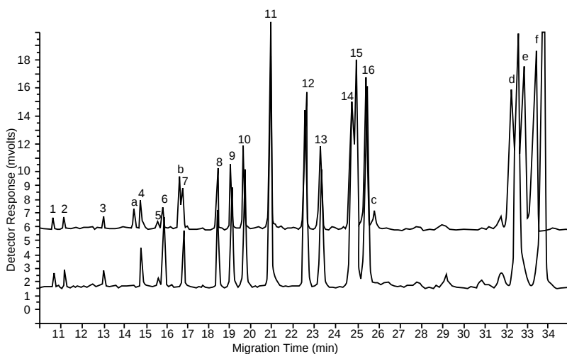
Figure 2-1. Comparison of N -glycanase-treated CHO cell-expressed (lower trace) versus E. coli expressed (upper trace) rHuEPO tryptic maps by HPCE. Reproduced with permission from Rush et al., Anal. Chem. 65, 1834 (1993).
