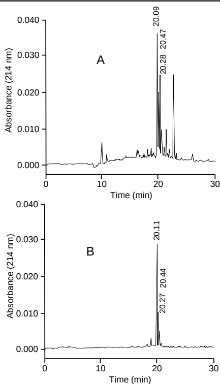
Figure 2-15. (A) Separation by CZE of an r-hirudin-containing sample from a fermentation broth. (B) Purified r-hirudin sample. Run buffer: 20 mM tricine, 10 mM sodium borate, 1 mM EDTA, 0.2 mM diaminobutane, pH 8.4. From Paulus and Gassman, Beckman Application Data Sheet DS-752.
