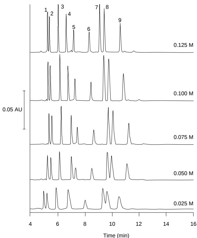
Figure 1-26. Effect of the buffer ionic strength on peak shape and migration time of peptides. Buffer: sodium phosphate, pH 2.44; 30 kV; 20 °C; 200 nm; 57 (50) cm \times 75 \mu m capillary. Peak identification: (1) dynorphin; (2) bradykinin; (3) angiotensin II; (4) TRH; (5) LHRH; (6) bombesin; (7) leu-enkephalin; (8) met-enkephalin; (9) oxytocin. From McLaughlin et al., Beckman Technical Information Bulletin TIBC-106 (1991).
