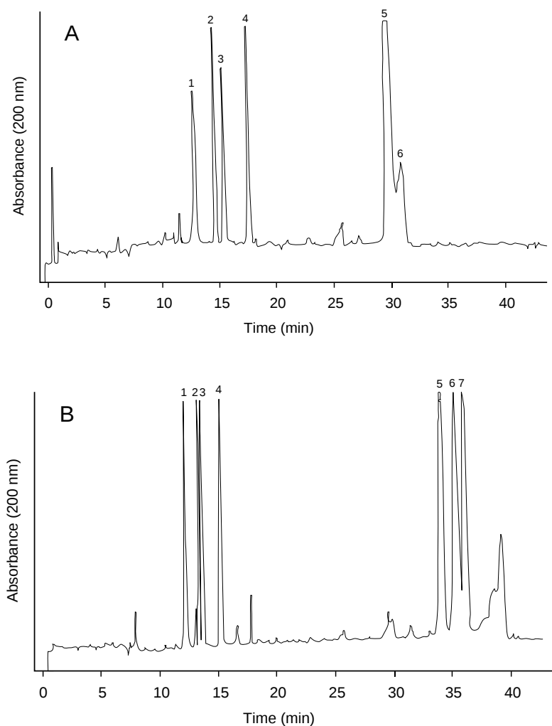
Figure 1-8. MECC of enkephalin analogs (A) without and (B) with the addition of 5% acetonitrile to the buffer. Capillary, 65 cm \times 75 \mu m, 100 mM sodium borate, 100 mM SDS, pH 8.5, 15 kV, 25°C, 200 nm. Peak identification: (1) metsulfoxide enkephalin; (2) methionine enkephalin; (3) [ala 2 ] methionine enkephalin; (4) leucine enkephalin; (5) leucine enkephalin amide; (6) leucine enkephalin-arg; (7) proenkephalin.
