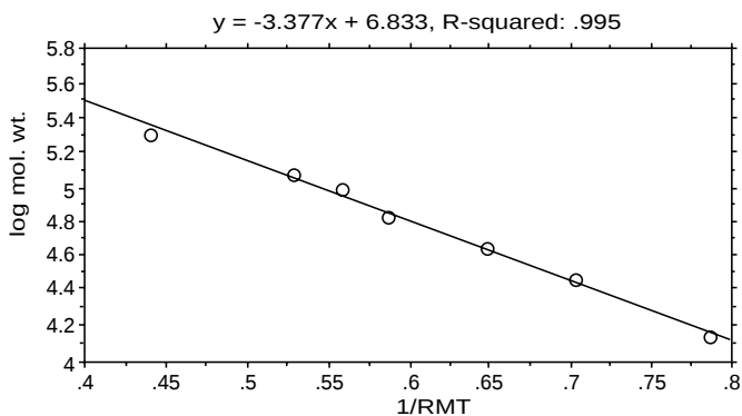
Figure 1-35. Molecular weight standard curve
