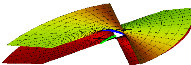
Figure 1. Oriented pair \{M, \widehat{M}\} with \widehat{\alpha}(r) blue, and \alpha(r) green.
