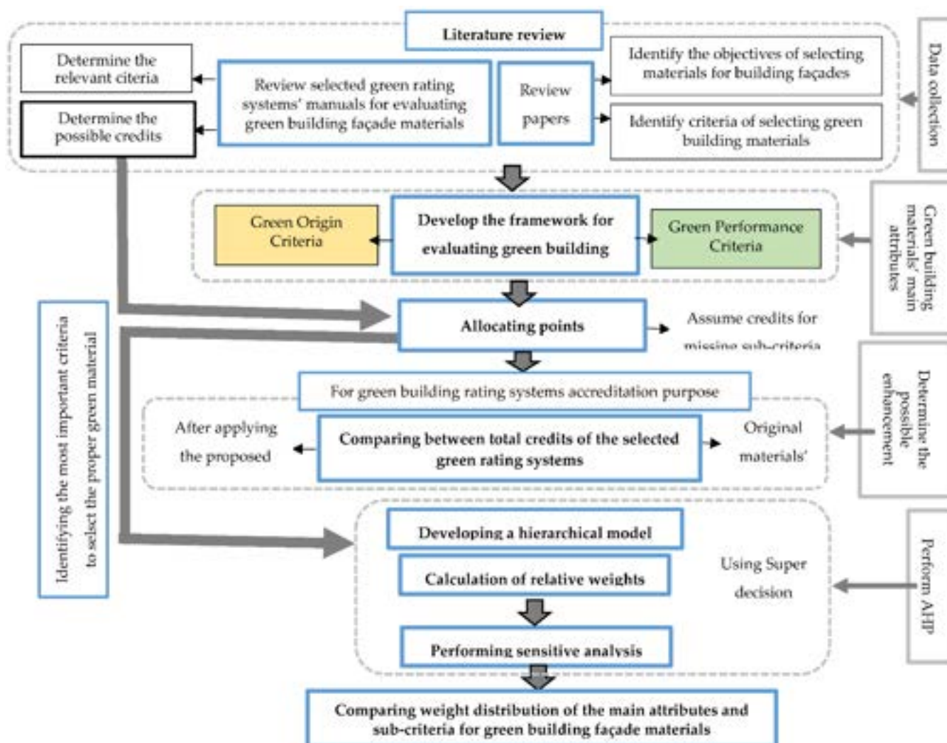
Figure 2. Research methodology.
