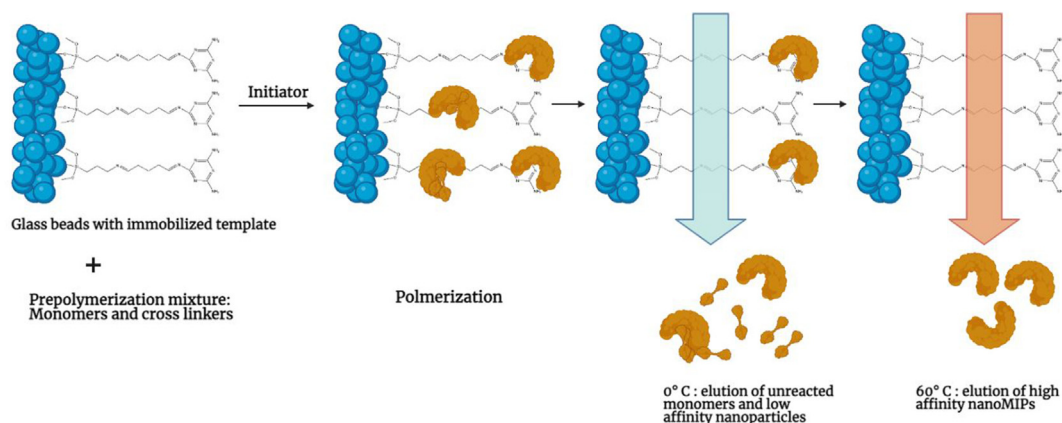
Fig. 4. Schematic illustration of solid phase synthesis of nanoMIPs. Prepolymerisation mixture is added to the column containing glass beads with immobilised template followed by initiation. Unreacted monomers and low affinity oligomers are eluted at low temperature. NanoMIPs are then eluted at higher temperature.
